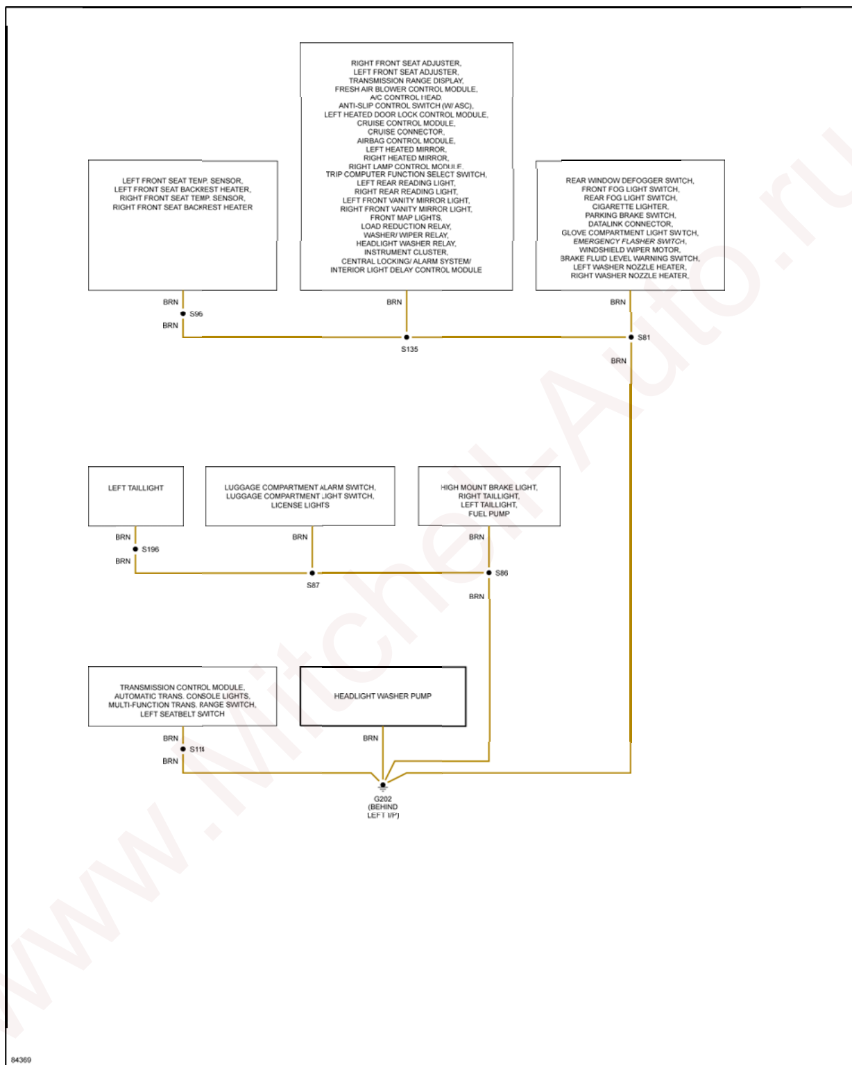
Fig. 17: Ground Distribution Circuit (2 of 2)
