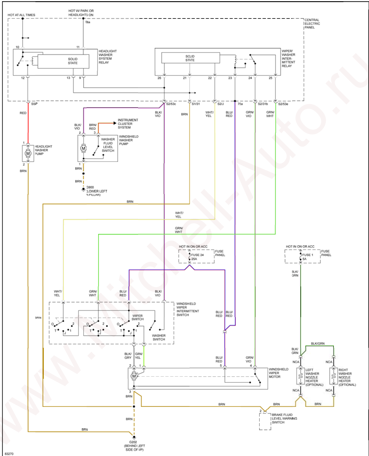
Fig. 39: Wiper/Washer Circuit
