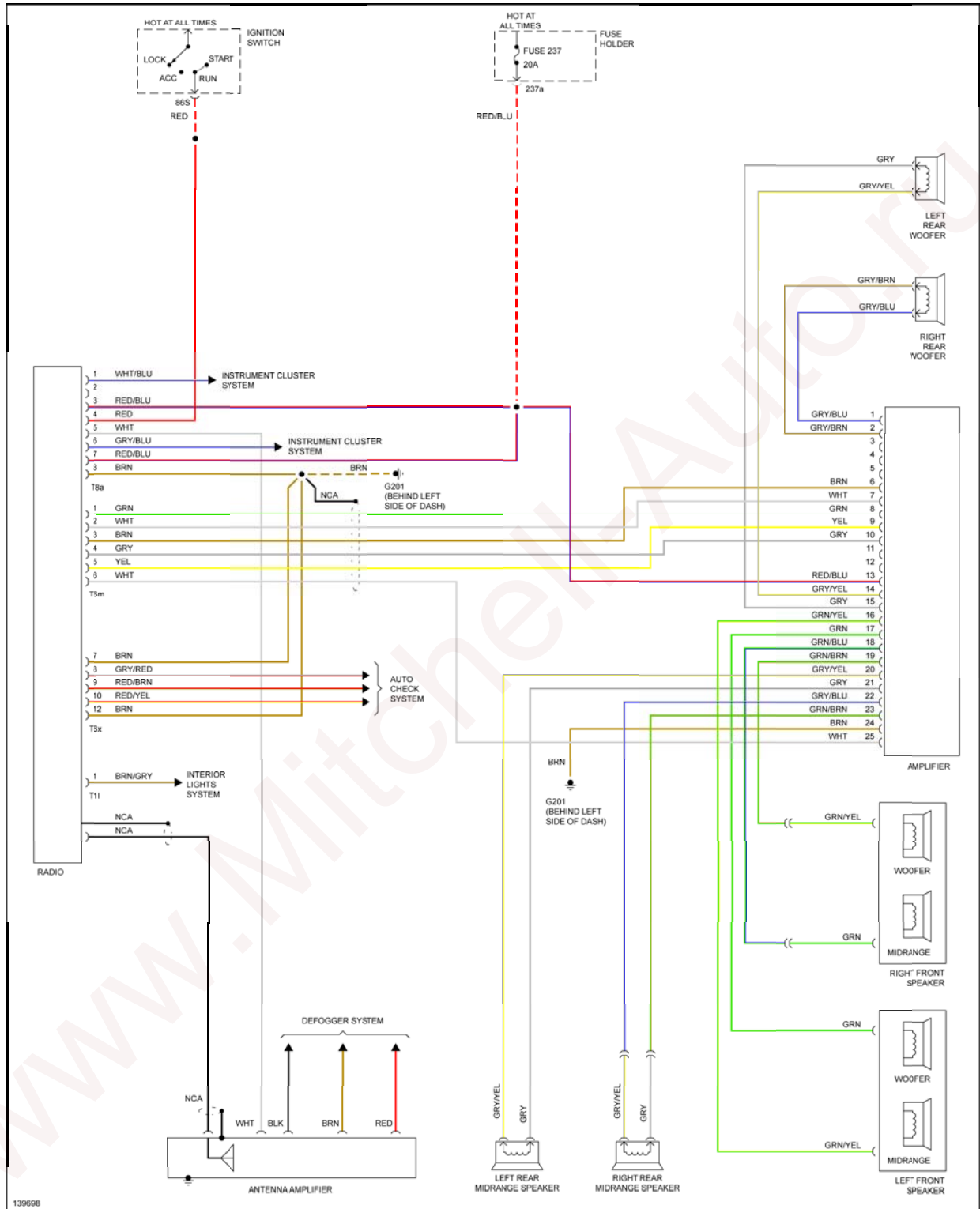
Fig. 32: Radio Circuit
